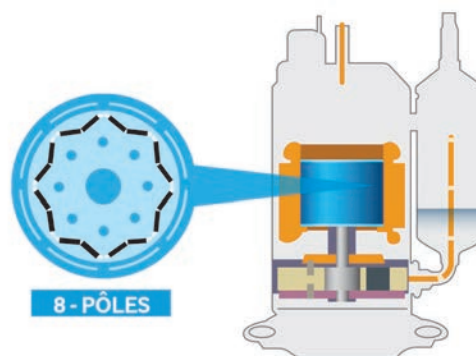
DIGITAL INVERTER 8-PÔLES
